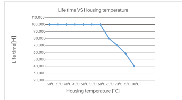
LA-30-200-1050-U1MA
