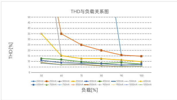
LA-30-200-1050-U1MA
