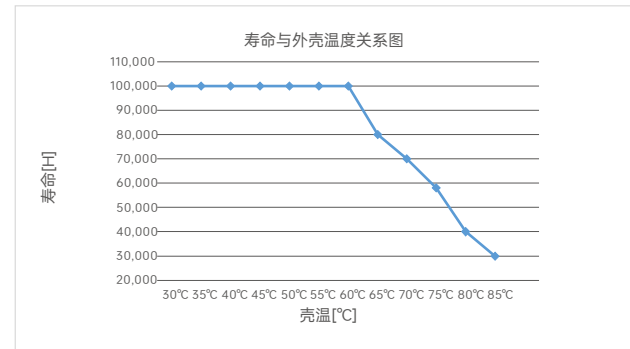
LA-40-300-1200-U1MA
