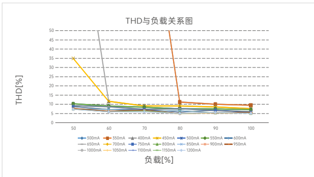
LA-40-300-1200-U1MA
