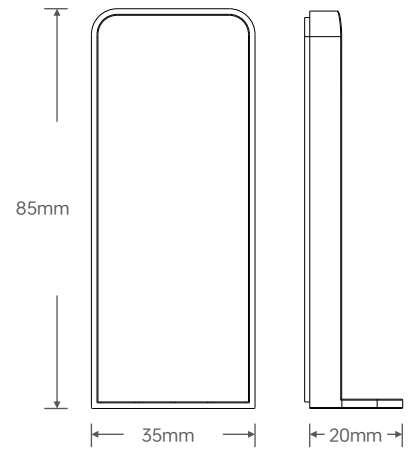
Magnetic Mount
