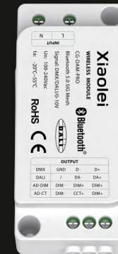
CG-DAM-PRO (三合一) 蓝牙 - DALI 0-10V DMX
